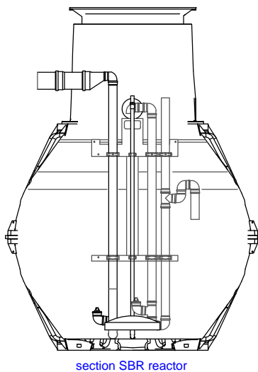
section SBR reactor
